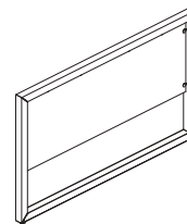
Close end leg with modesty 40x40x1.2 mm
