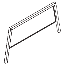
Slant end leg with modesty 40x40x1.2 mm
